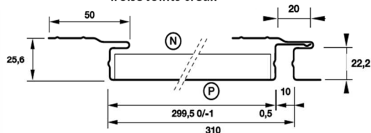
Iroise Joints creux
