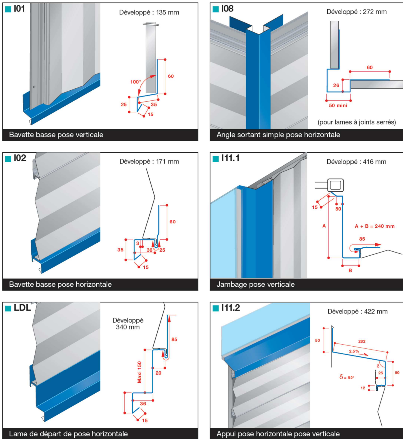
Figure 03 – Planche accessoires n°1
