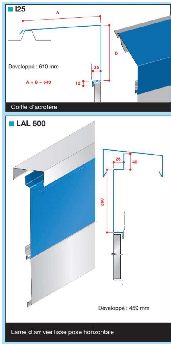
Figure 08 – Planche accessoires n°6
