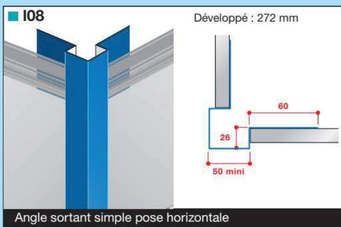
Figure 04 – Planche accessoires n°2
