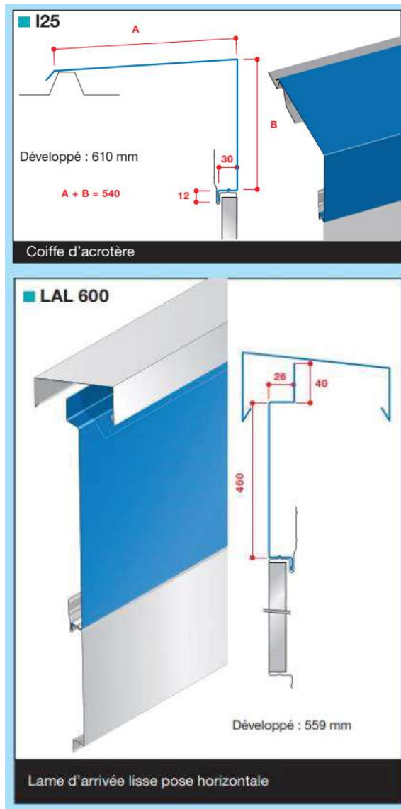
Figure 08 – Planche accessoires n°6
