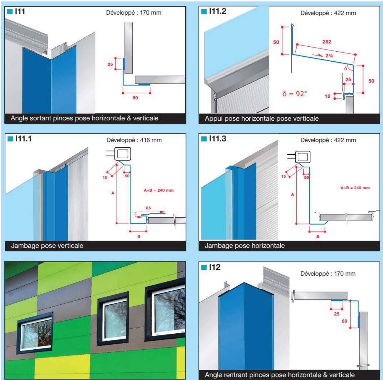
Figure 05 – Planche accessoires n°3
